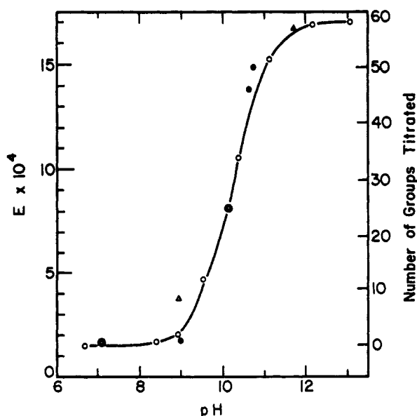
Fig. 8.—Spectrophotometric titration curve of paramyosin in GU-0.3 M KCl at 25° and at a wavelength of 295 mμ. The symbols have the same meaning as in Figure 7.
