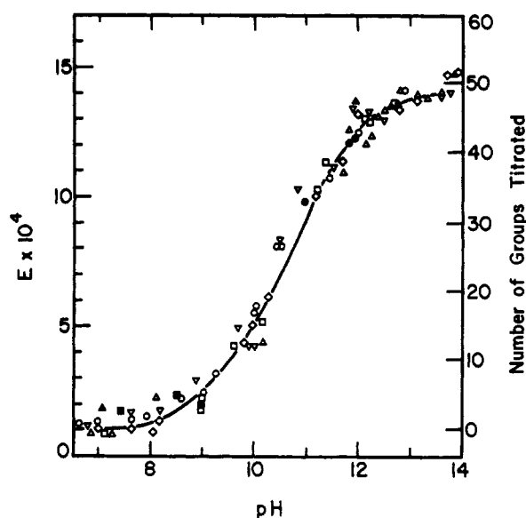
Fig. 7.—Spectrophotometric titration curve of paramyosin in 0.3 M KCl at 25° and at a wavelength of 295 mμ. The symbols of various types denote separate experiments. The closed symbols represent the reverse titration.
